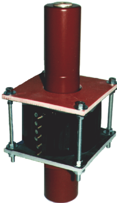
PIBCT CT & Bushing Assembly Flanged Bushing with PRCT05 CT and GPO Mounting
